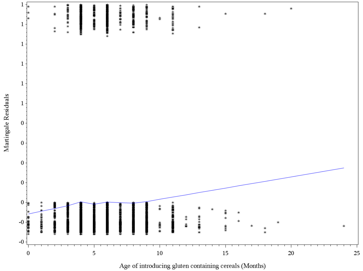
Supplementary Figure 1. Martingale residuals for timing of introducing gluten containing cereals and the risk of any IA retrieved from the unadjusted Cox regression model.
